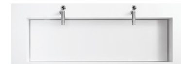
63" E052463-1D-A01 (double single faucet hole) Matte white (A01) solid surface W 63" (160cm) x D 19-5/8" (50cm) x H 7-1/8" (18cm)
